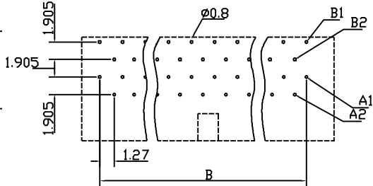
P.C. Board Layout Top View (26,34,50 Position)
