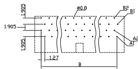
P.C. Board Layout Top View (20,32,40,52,60,68,80,100 Position)
